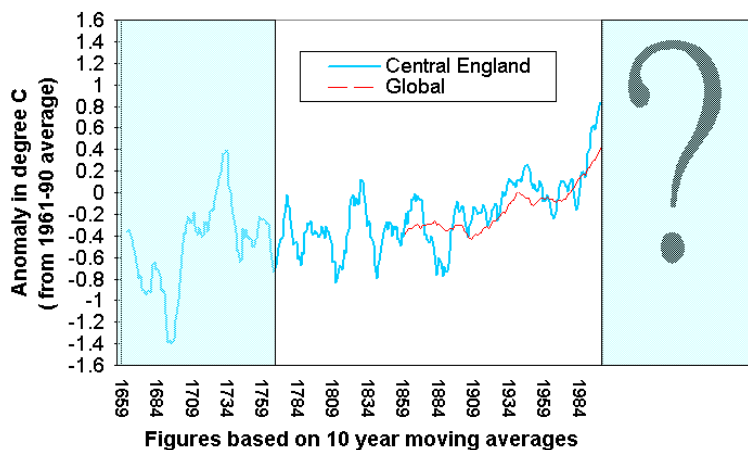
Central England & Global surface temperature anomalies 1663 to 2100
